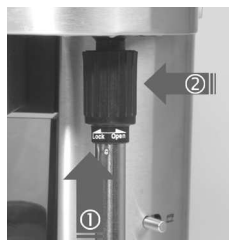
① Touch the stainless steel nozzle at the shaft for attaching it and push the nozzle on. ② Then, turn it to the left and lock it.
